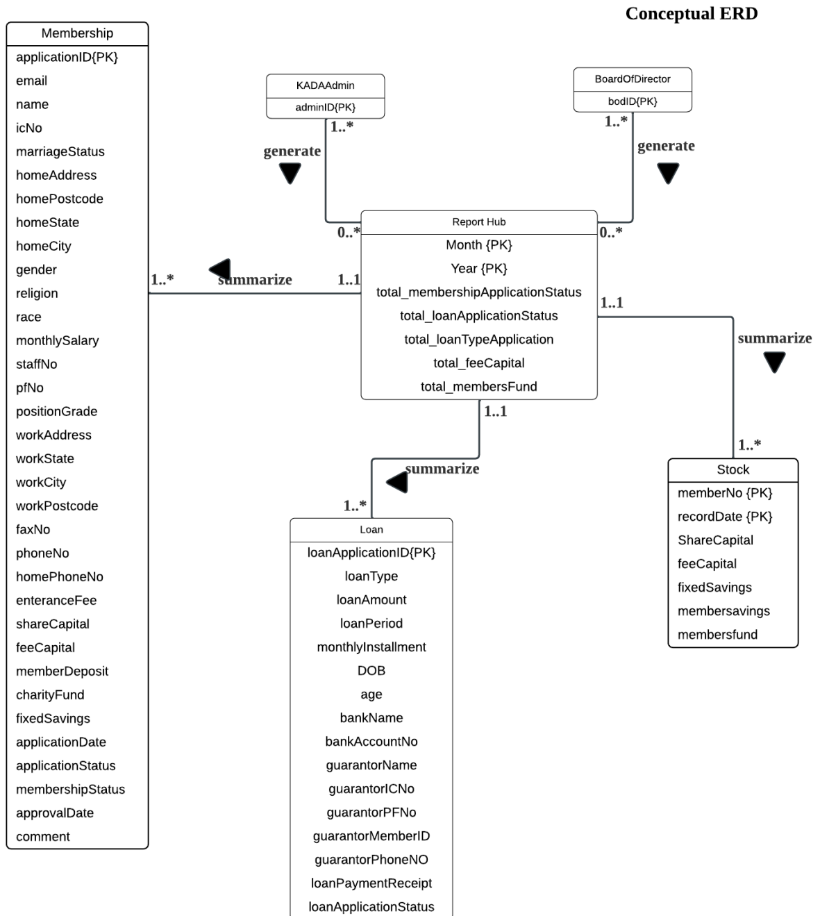
Figure 2.1.1 Conceptual ERD of Report Hub Module
