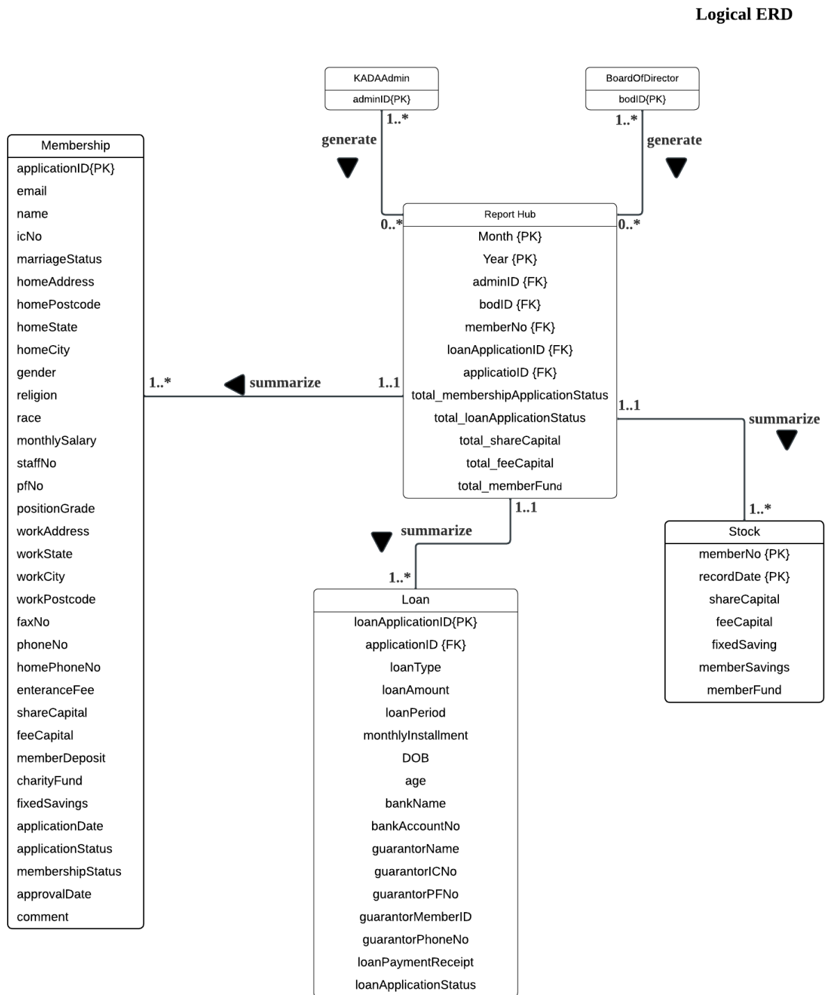
Figure 2.1.2 Logical ERD of Report Hub Module
